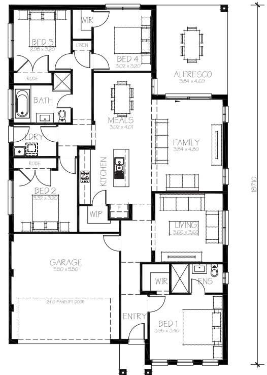
FLOOR PLAN
